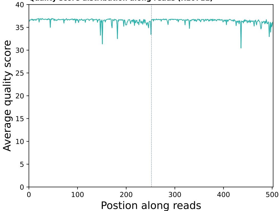
Quality score distribution along reads (R10711)
